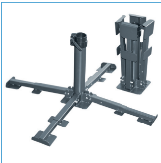
Plate stand foldable, ~ 6 kg Pole diameter: Ø 50-55 mm Conc. plates: 40x40/50x50 cm Color: anthracite Article Number: 490804
